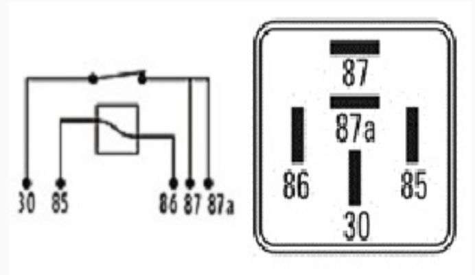
DIAGRAMA DIMENSIONAL
