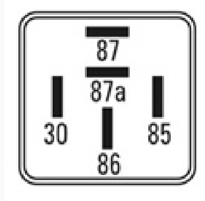
DIAGRAMA DIMENSIONAL
